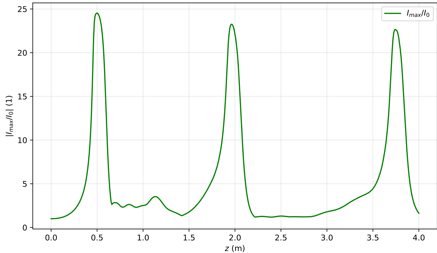
I_{\max}(x=0, y=0, z)/I_0 , Pin=9.0Pcr, artificial time
